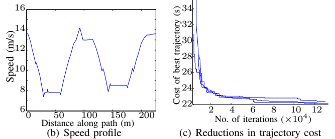
Fig. 5. Motion planning with the half-car model over a closed circuit.
