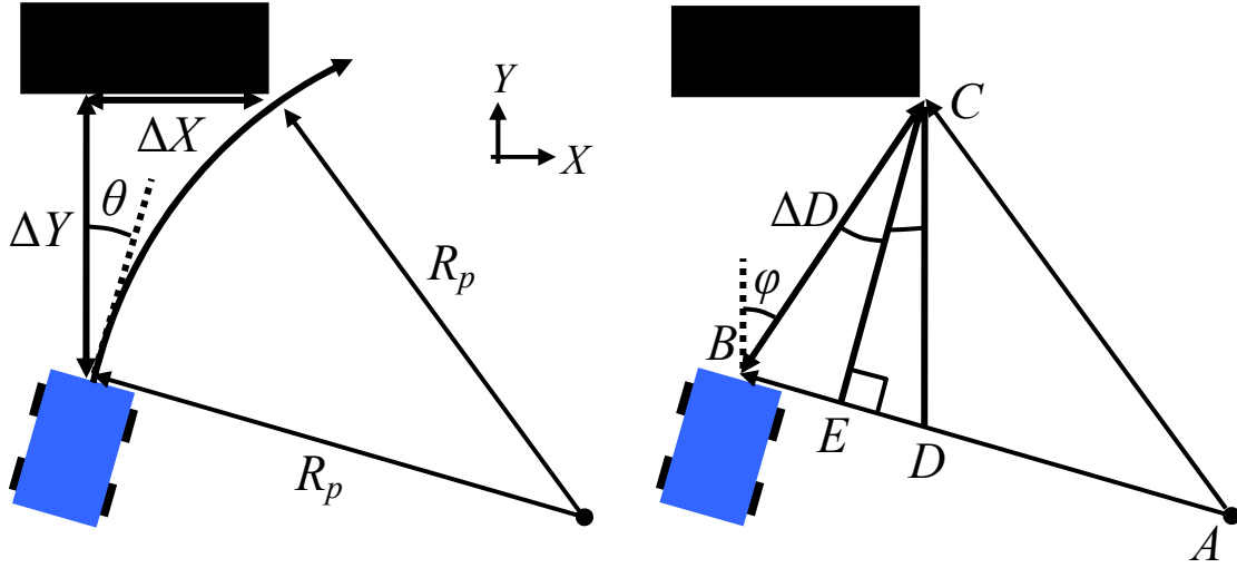
Fig. 3.5: Geometry of passing turn to the right.
