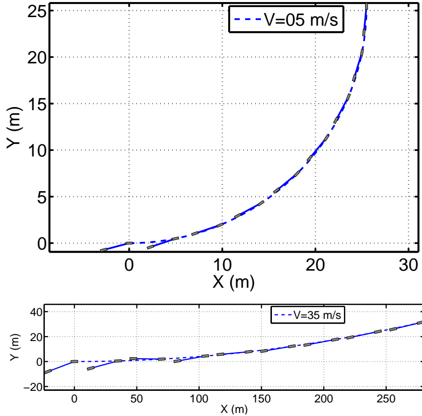
Fig. 4.13. Snapshots at 1 second intervals of vehicle orientation while tracking steady turning trajectories at constant speed with u_{\theta 3} = 0.1 and u_3=0 . The vehicle size is enlarged and not to scale in the illustration of the 35 m/s trajectory to improve visibility.
