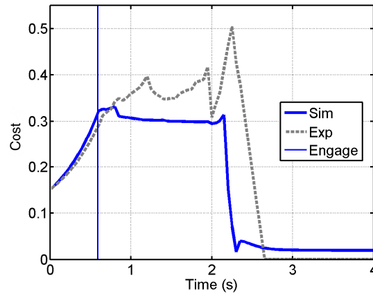
Fig. 5.15: Predicted cost during passing turn at 13 m/s with \Phi_{on} = 0.3 .
