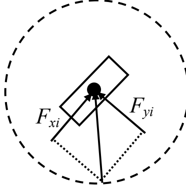
Fig. 2.3: Illustration of friction circle constraint.
