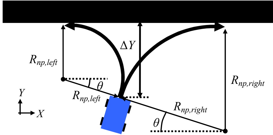
Fig. 3.4: Geometry of non-passing turns.
