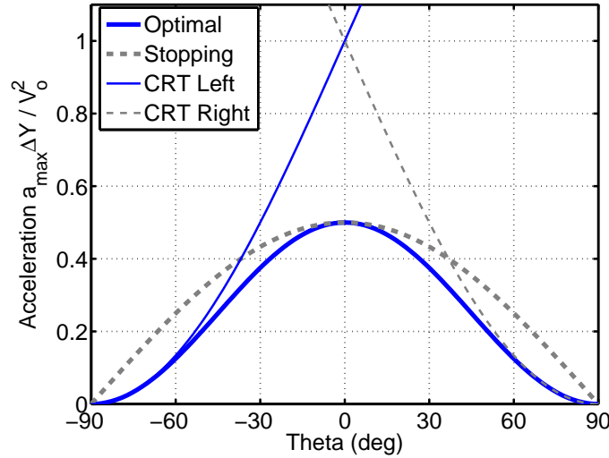
Fig. 3.10: Comparison of non-passing and stopping maneuvers.
