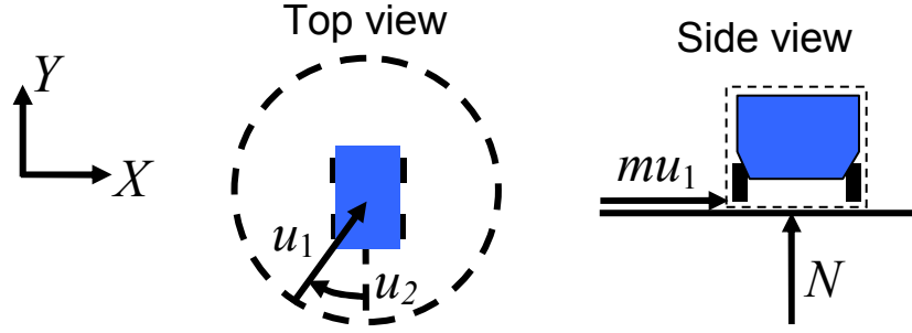
Fig. 3.1: Point mass with acceleration circle constraint.
