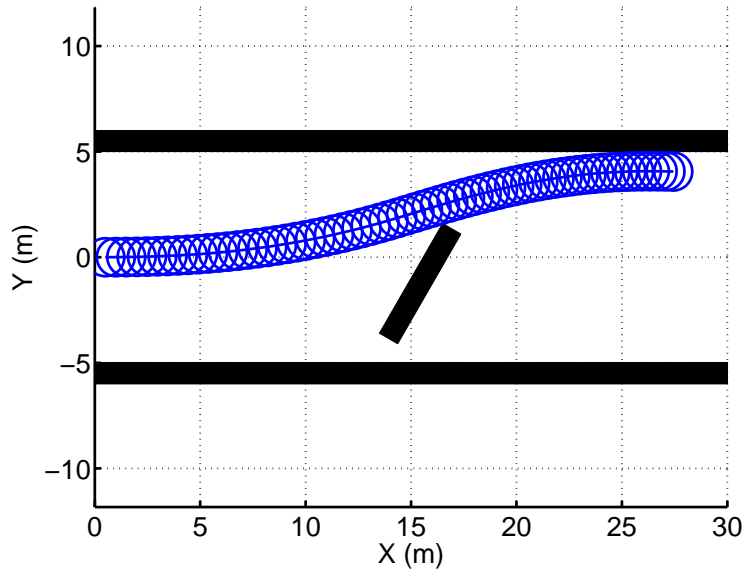
Fig. 2.6: Optimal trajectory computed numerically
