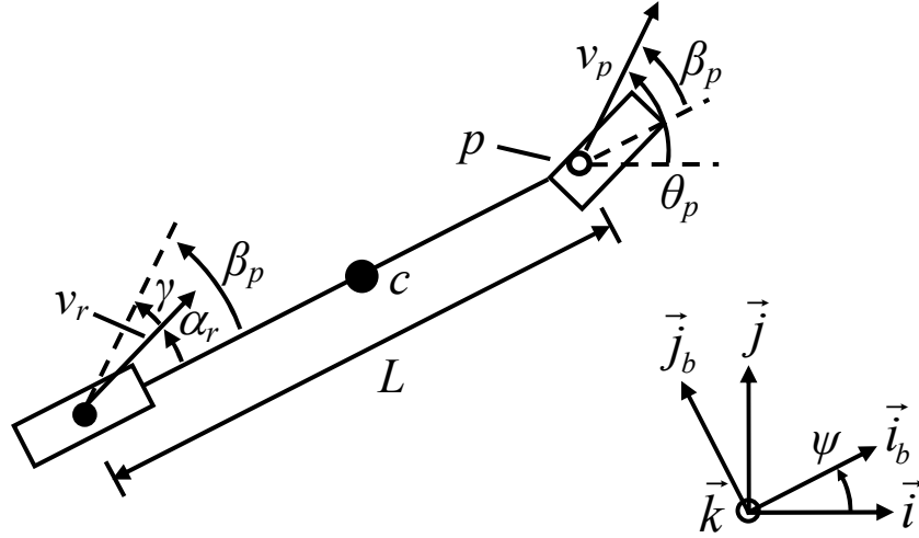
Fig. 4.2: Nonlinear bicycle model with front center of oscillation and rear wheel marked.
