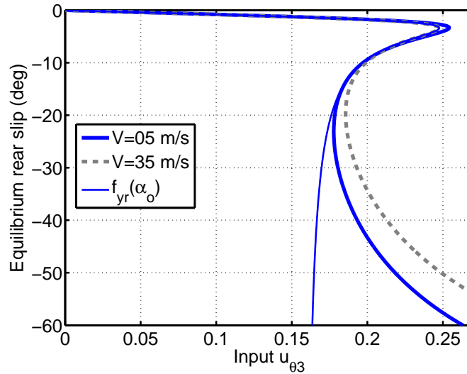
Fig. 4.9. Plots of equilibrium rear slip \alpha_o for a given value of u_{\theta 3} computed numerically from (4.120) for v_p = 5 m/s and v_p = 35 m/s. The curve corresponding to u_{\theta 3} = f_{yr}(\alpha_o) is plotted as well for reference.
