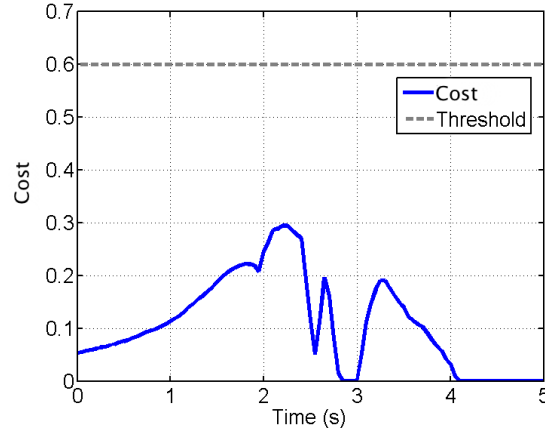
Fig. 5.13: Predicted cost during passing maneuver initiated by driver without intended controller intervention.
