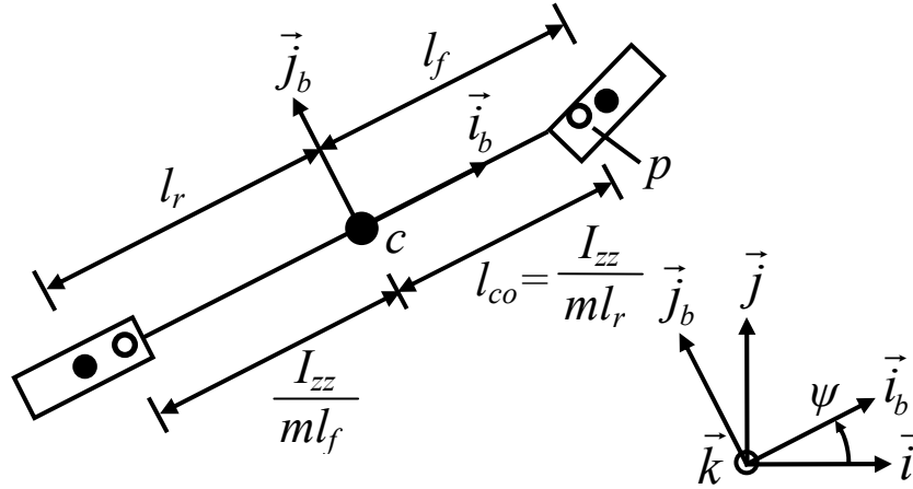
Fig. 4.1: Nonlinear bicycle model with wheel centers marked as solid circles and centers of oscillation as hollow circles. The front center of oscillation is marked as point p .
