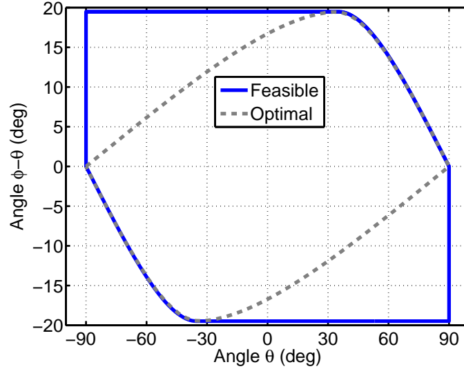
Fig. 3.18: Range of angles \varphi-\theta for which the optimal passing maneuver is feasible (Feasible) and requires less acceleration than optimal non-passing (Optimal).
