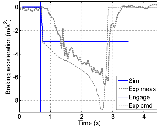
Fig. 5.11: Vehicle braking acceleration during stopping maneuver at 8 m/s with \Phi_{on} = 0.3 . The simulated acceleration is denoted by "Sim" and the commanded and measured accelerations from the experiment are denoted "Exp cmd" and "Exp meas" respectively.
