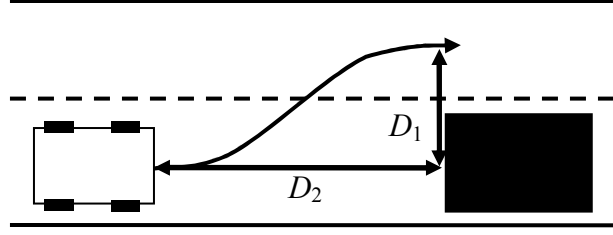
Fig. 1.2: Lane change maneuver.
