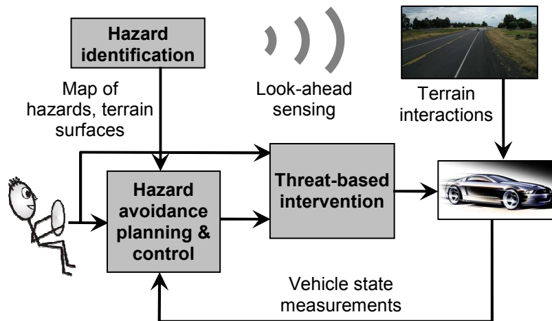
Fig. 5.1: Semi-autonomous hazard avoidance system design.
