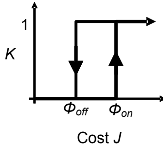
Fig. 5.5: Switching intervention law with hysteresis.
