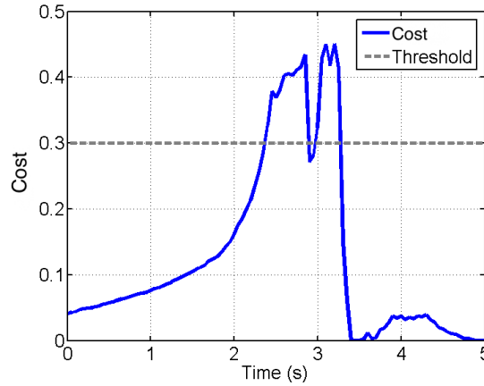
Fig. 5.19: Predicted cost during non-passing turn maneuver initiated by controller intervention.
